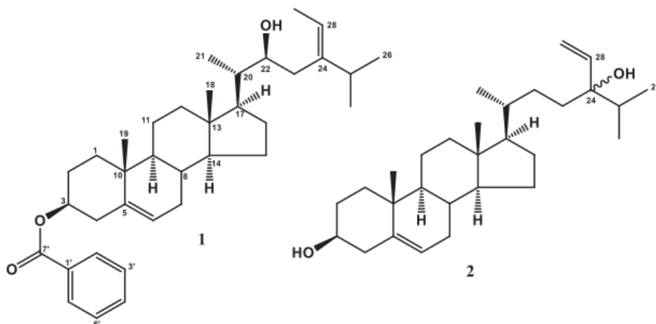
Figure 1. Structures of Compounds 1–2.
