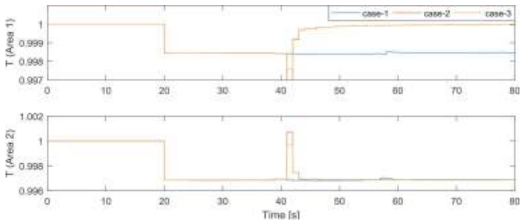
Figure 22. Time constant T of IMC type 1.
