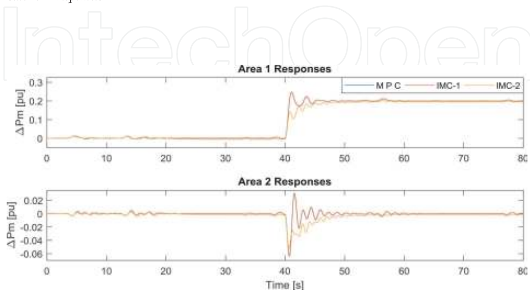
Figure 18. Case 2: \Delta P_m responses.
