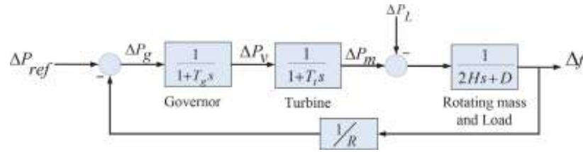
Figure 6. Completed power system block diagram.
