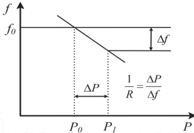
Figure 4. Speed drop regulation.
