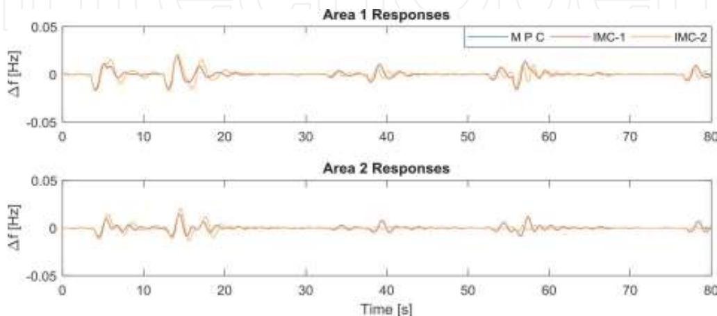
Figure 15. Case 1: \Delta f responses.
