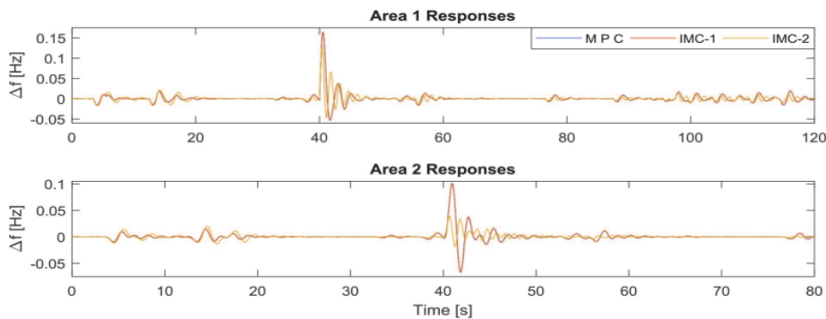
Figure 19. Case 3: \Delta f responses.
