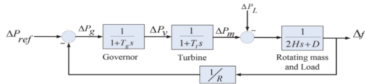
Figure 6. Completed power system block diagram.
