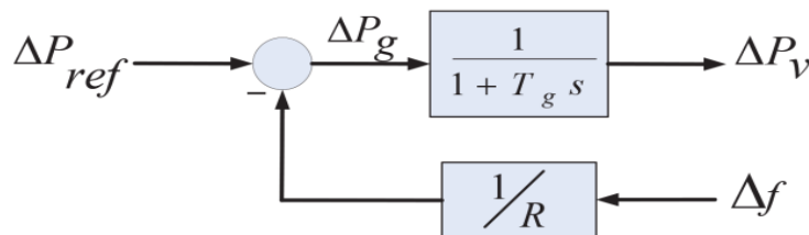
Figure 5. Block diagram for governor.
