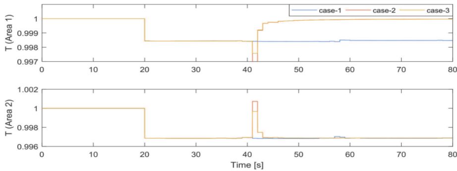
Figure 22. Time constant T of IMC type 1.
