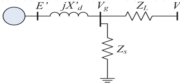
Figure 8. Single machine system.
