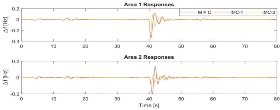
Figure 17. Case 2: \Delta f responses.
