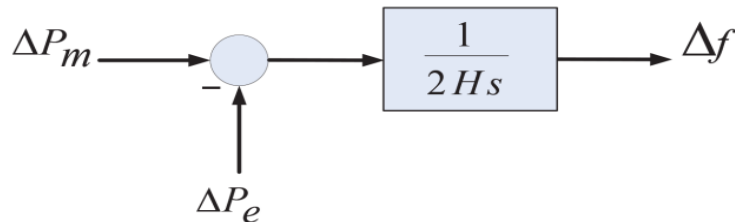
Figure 1. Block diagram for generator.
