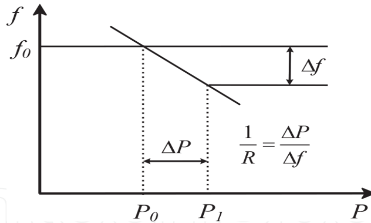
Figure 4. Speed drop regulation.
