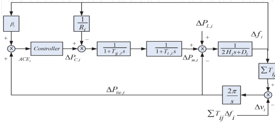
Figure 7. Power system dynamics.
