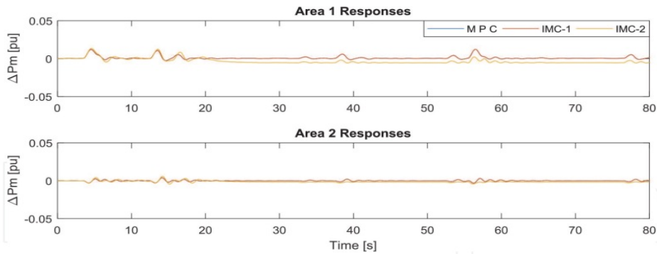
Figure 16. Case 1: \Delta P_m responses.
