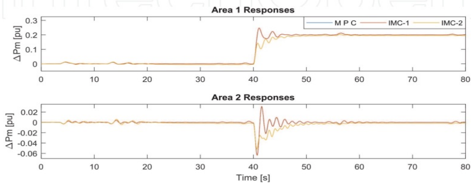
Figure 18. Case 2: \Delta P_m responses.
