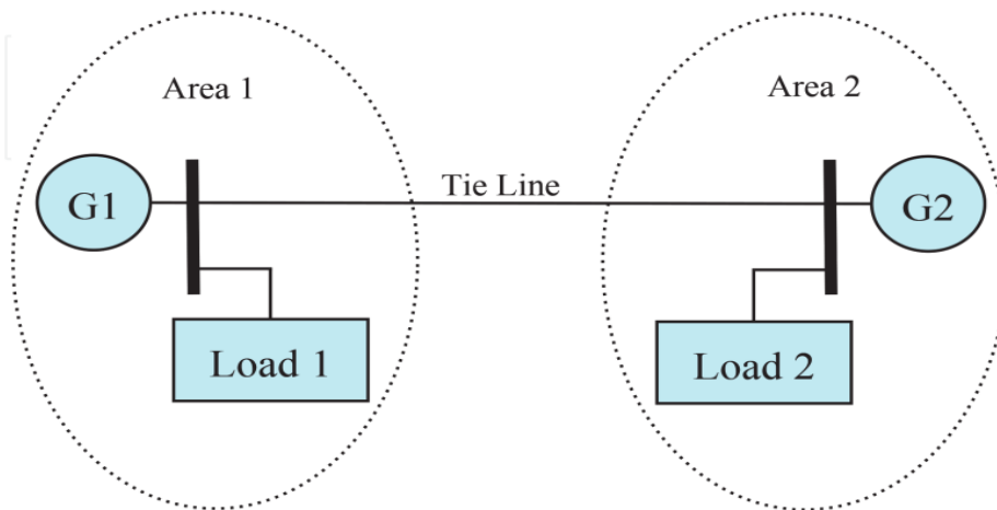
Figure 14. Multi-area power system configuration.
