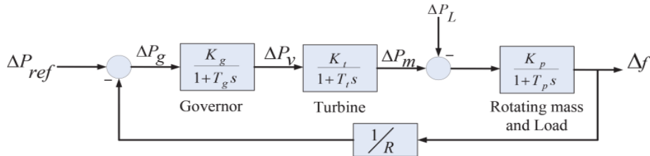
Figure 11. Power system model.
