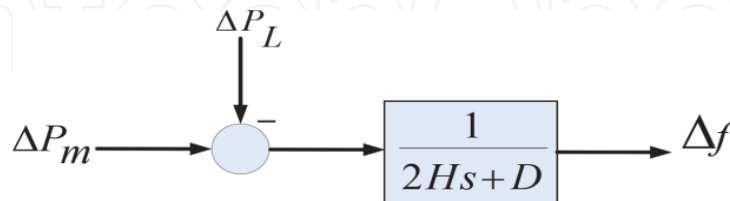
Figure 2. Generator and load block diagram.
