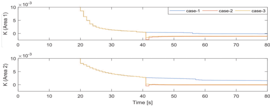
Figure 23. Gain K of IMC type 2.
