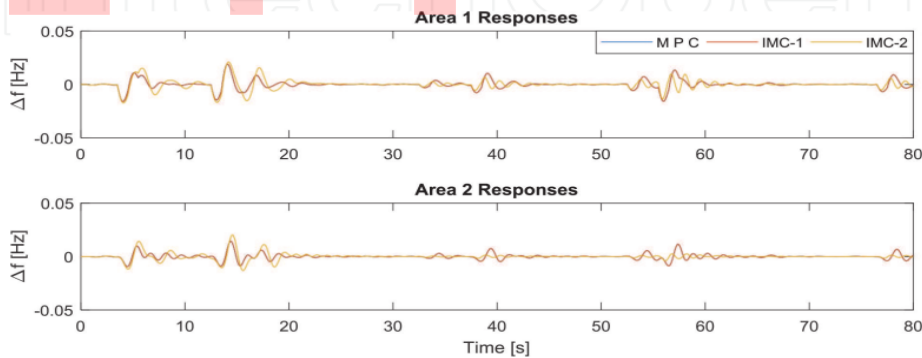
Figure 15. Case 1: \Delta f responses.
