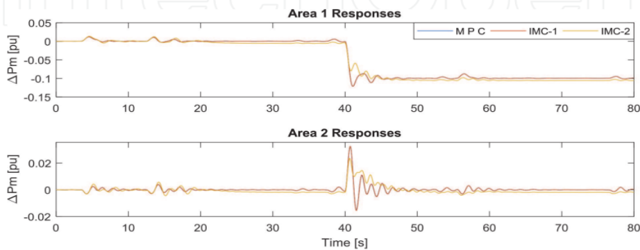
Figure 20. Case 3: \Delta P_m responses.
