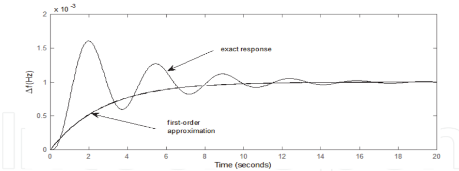
Figure 12. First- and third-order system responses.
