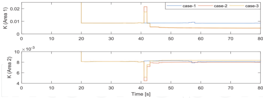
Figure 21. Gain K of IMC type 1.
