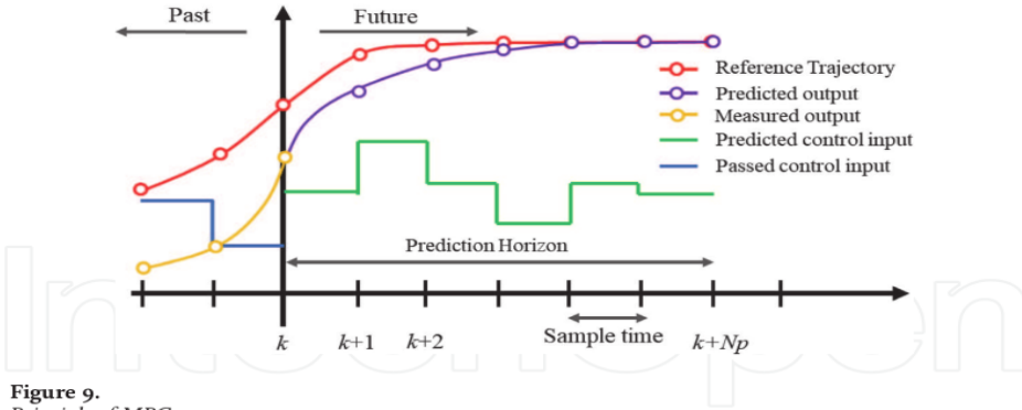
Figure 9. Principle of MPC.
