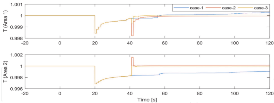
Figure 24. Time constant T of IMC type 2.
