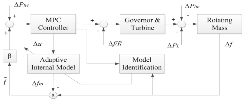
Figure 13. Adaptive LFC system using IMC structure.
