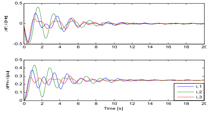
Fig. 5. Adaptive IMC-MPC controller responses in case I
