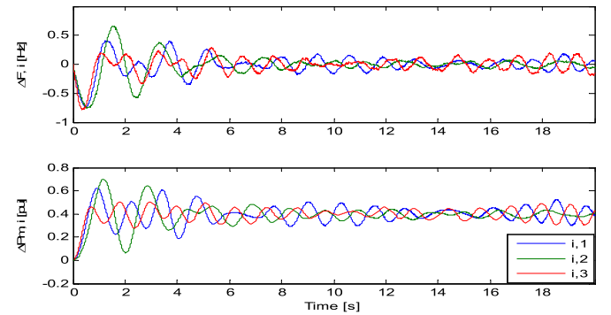
Fig. 7. Adaptive IMC-MPC controller responses in case II
