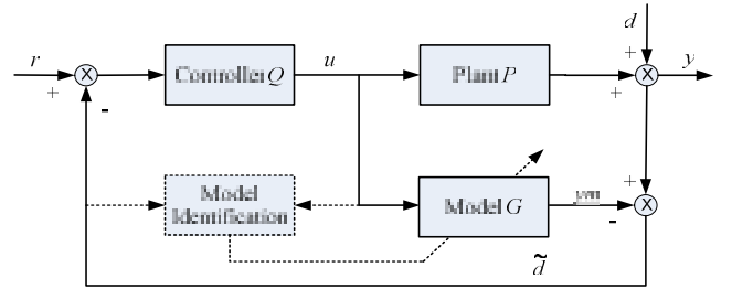
Fig. 1. IMC Principle
