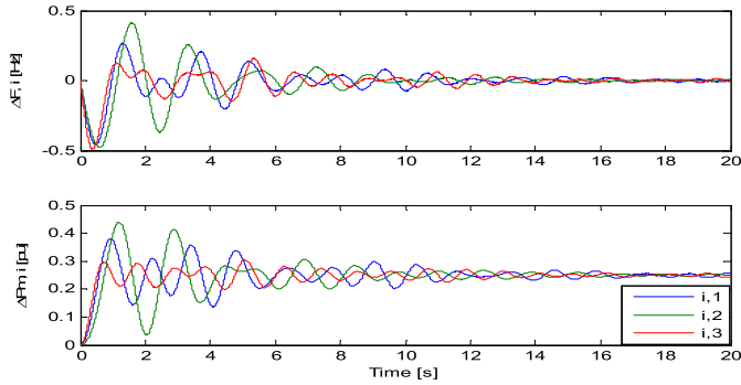
Fig. 9. Adaptive IMC-MPC controller responses in case III
