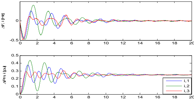
Fig. 4. MPC controller responses in case I
