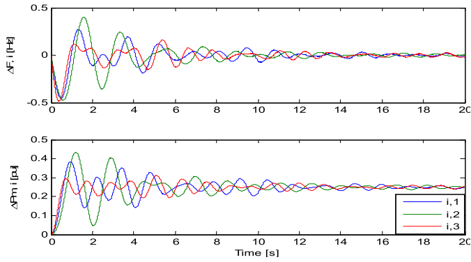
Fig. 8. MPC controller responses in case III
