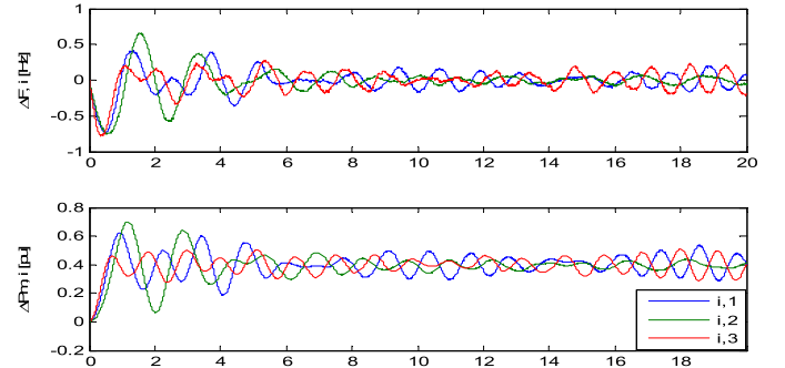
Fig. 6. MPC controller responses in case II
