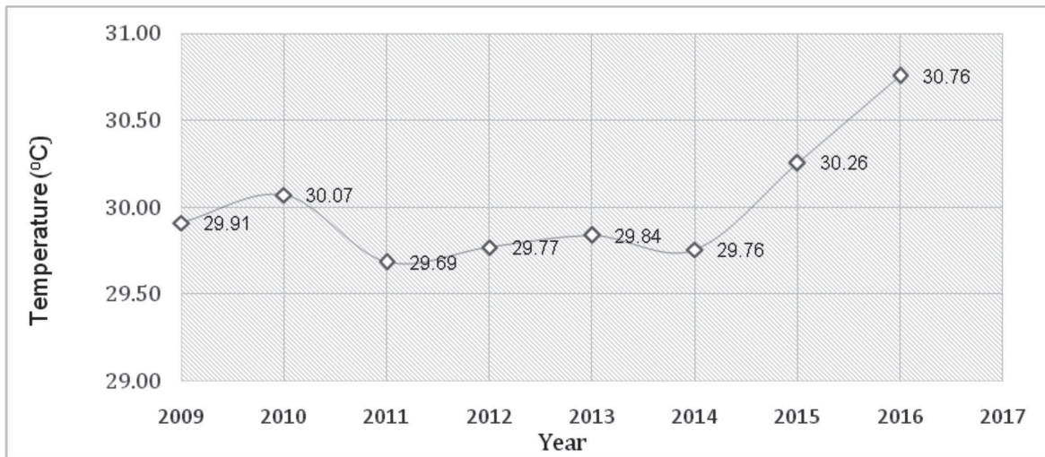
Fig. 5. Trends of sea surface temperature in the period of time between 2009 and 2016 (Aviso, 2016)
