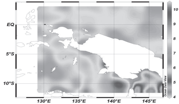
Fig. 2. Sea level rise in Papua and Raja Ampat coastal area
