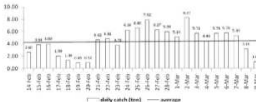
Figure 3. Temporal distribution of oil sardine production taken from the Bali Strait in February-March 2015.
