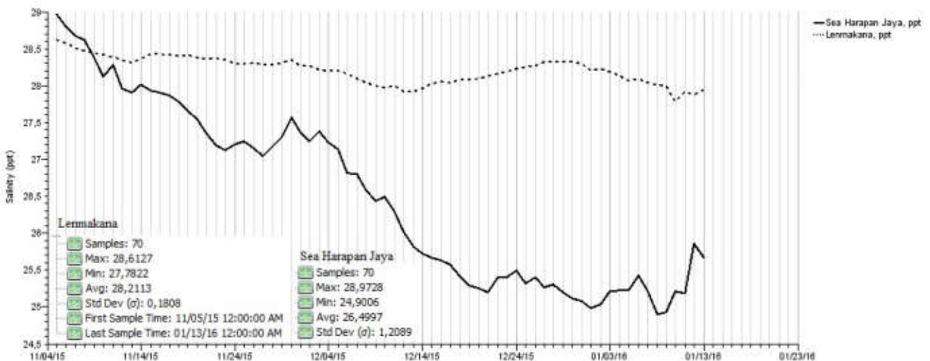
Figure 7. Time series of salinity at Sea Harapan Jaya and Lemakana Lake at Misool karst islands, Raja Ampat, West Papua. The loggers were installed at 3.5 m and 2.5 m, respectively. Data points were the daily averages from 24 hours of data recording
