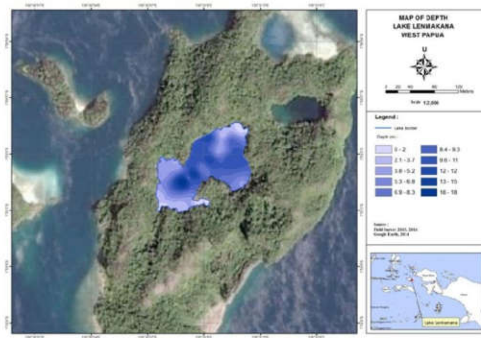
Figure 2. Bathymetry of Lemmakana Lake, Misool karst islands, Raja Ampat, West Papua
