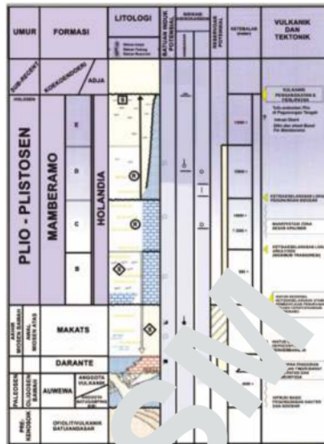
Gambar 3. Stratigrafi Cekungan Papua U (Shell, 1985; Waschsmuth & Kunst, 1986; Mcadams & Heibig, 1995; Grogan, 2005).
