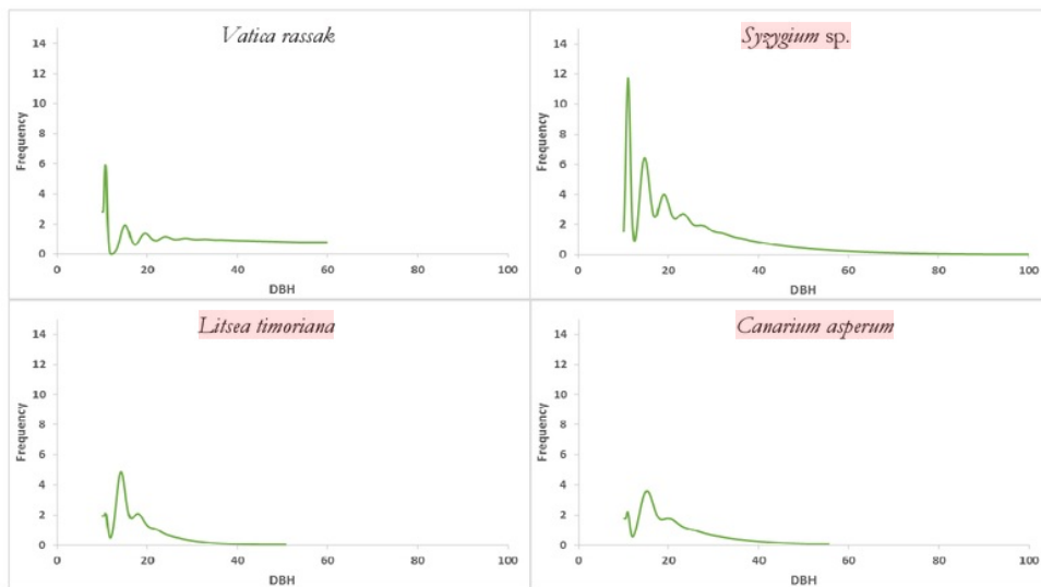
Figure 2. Stand structures with stable population of four species in logged forest. The stand structures were illustrated by plotting frequencies of individual trees over each diameter (cm) and n=500 number of matrices in simulation of IPMs when \lambda was stable
