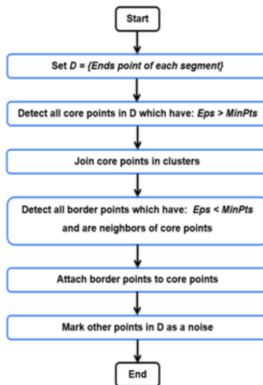
Fig. 2: Flowchart of DB –Scan
