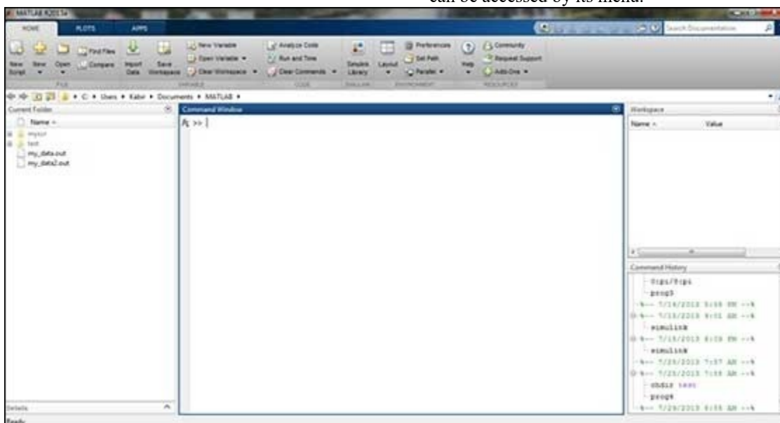
Fig 3: MATLAB environment
