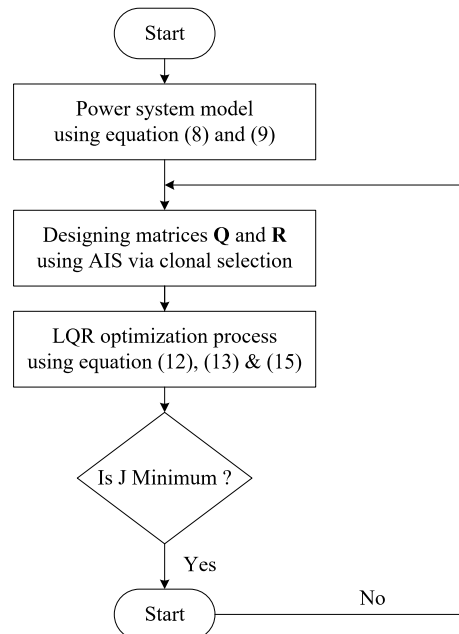
Figure 7. Proposed method
