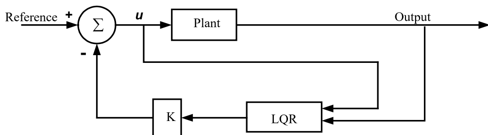
Figure 4. Block diagram control system
